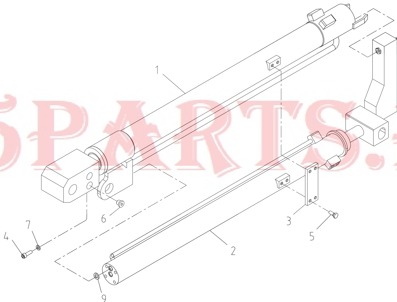
Fig. 1-1 SCS513 TELESCOPIC CYL' ASS'Y
