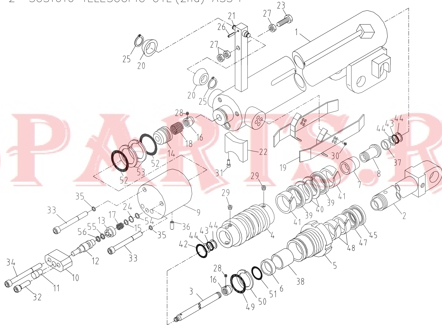
Fig. 1-1-2 SCS1616 TELESCOPIC CYL'(2nd) ASS'Y
