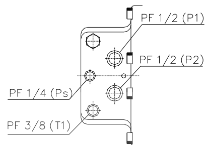
Fig. 2-1 SCS1015LSuper 2 SPEED WINCH ASS'Y
