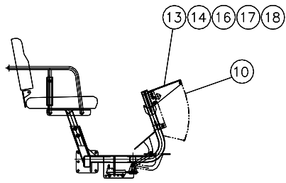
TOP SEAT
