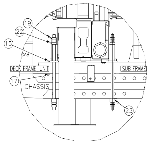
DETAIL D
